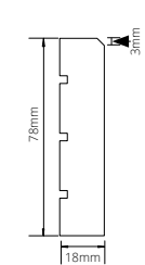
CONTEMPORARY ARCHITRAVE 78 x 18mm
