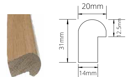
OAK HOCKEY STICK 20mm x 31mm
