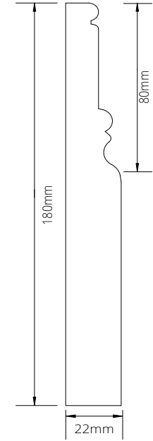
GRANGE SKIRTING 180(H) x 22(W) x 4200mm(L)
