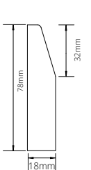
CHAMFERED ARCHITRAVE 78 x 18mm
