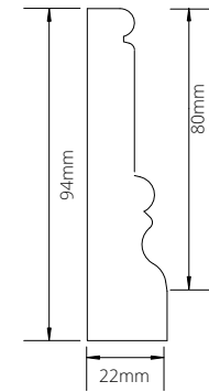
GRANGE ARCHITRAVE 94(H) x 22(W) x 2200mm(L)
