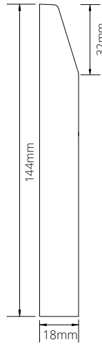
CHAMFERED SKIRTING 144(H) x 18(W) x 4200mm(L)
