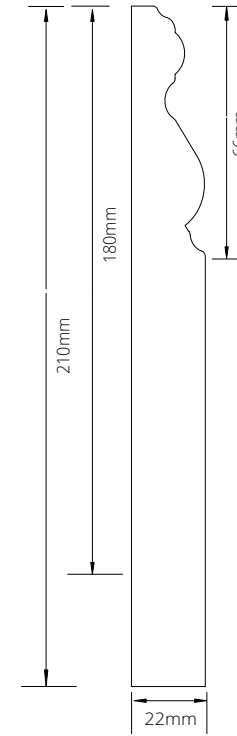
VICTORIAN SKIRTING 180/210(H) x 22(W) x 4200mm(L)
